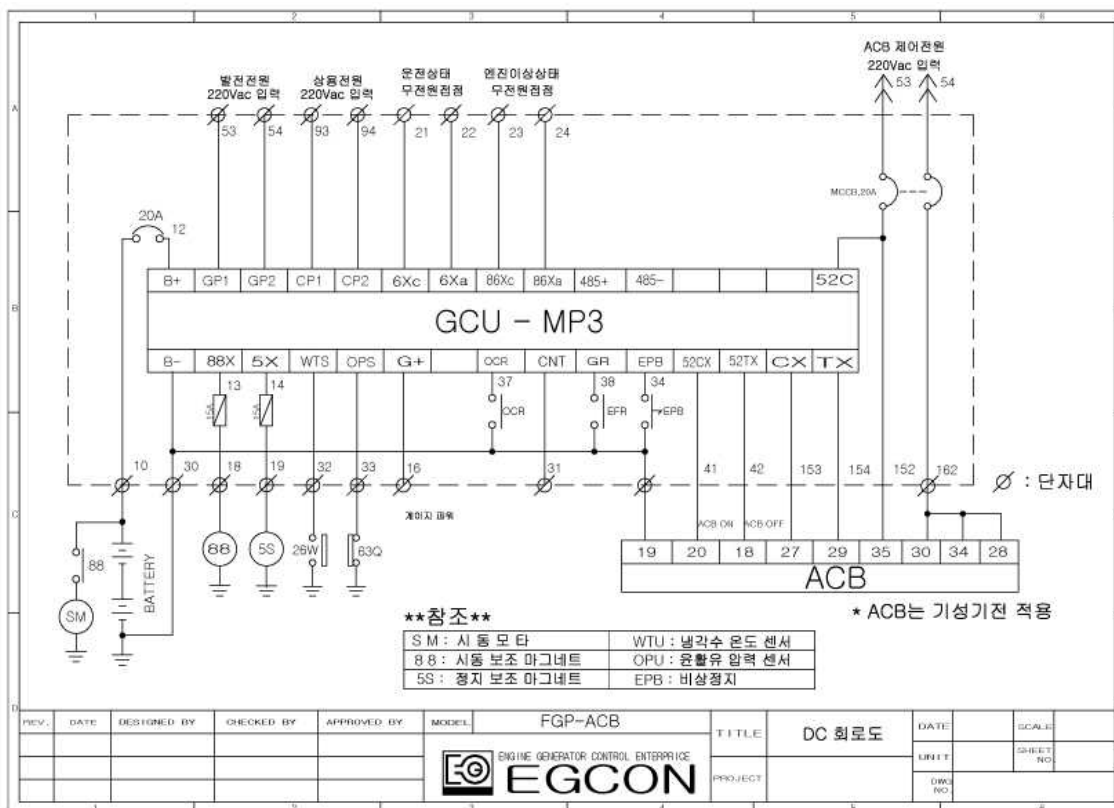
[회로도]
